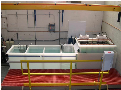
UNIGLO 500 Electro-Polishing/Passivation Processing System: Eliminates Chemical Replacement and No Waste Treatment Requirements
